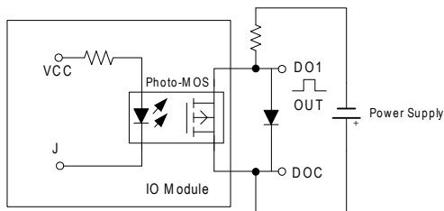
Figure 2-8 schematic diagram of digital output circuit 1
