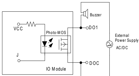
Figure 2-9 schematic diagram of digital output circuit 2
