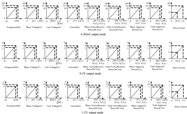
Figure 3-9 Relationship between analog output and various electrical quantities
