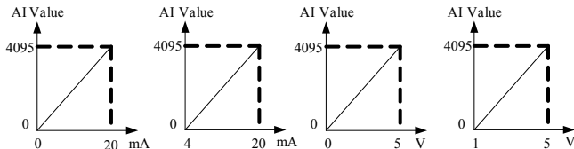
Figure 3-12 relationship between AI value and input analog value
